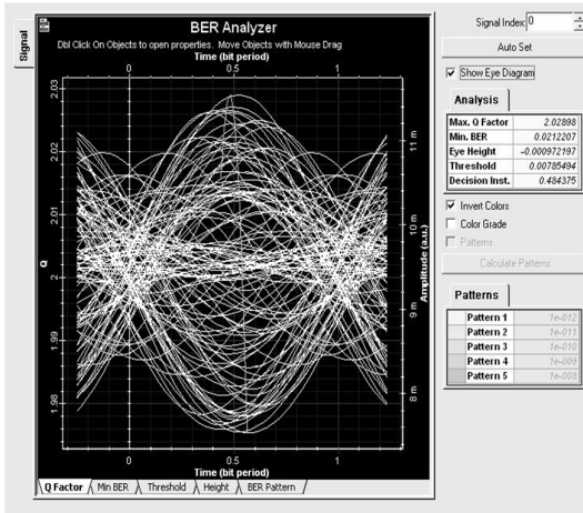
Fig 3(a). BER Analysis for ROF using MSK
