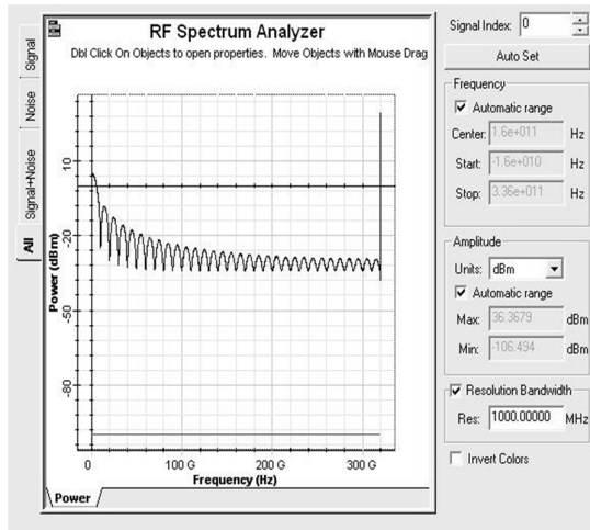
Fig 4(c). RF Spectrum Analysis for ROF using OQPSK
