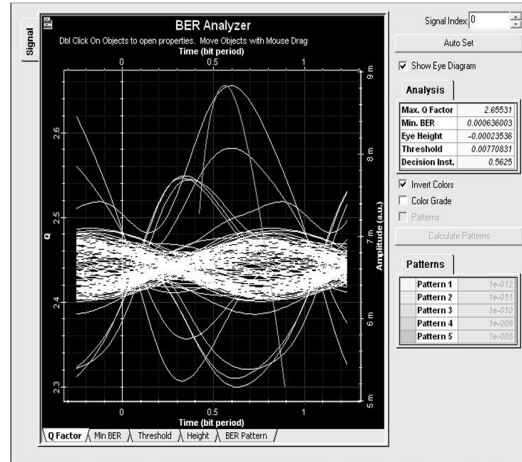
Fig 3(b). BER Analysis for ROF using DPSK
