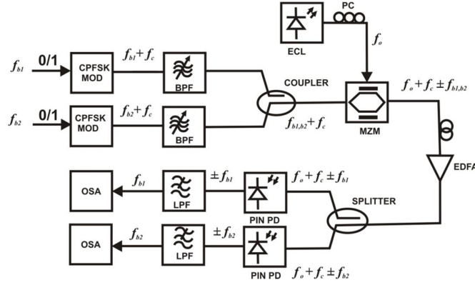
Fig 2(d). ROF Modulation using CPFSK
