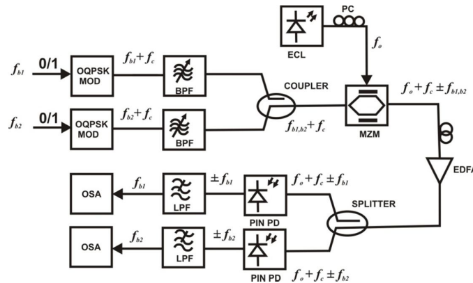
Fig 2(c). ROF Modulation using OQPSK
