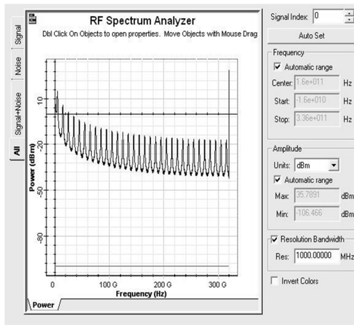
Fig 4(a). RF Spectrum Analysis for ROF using MSK
