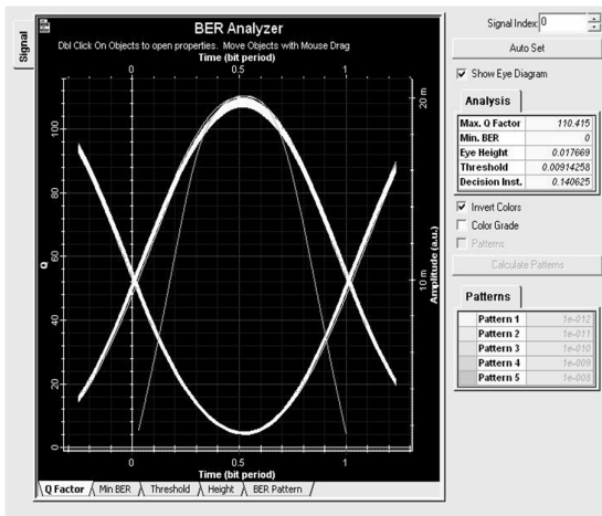
Fig 3(e). BER Analysis for ROF using Q-CPFSK
