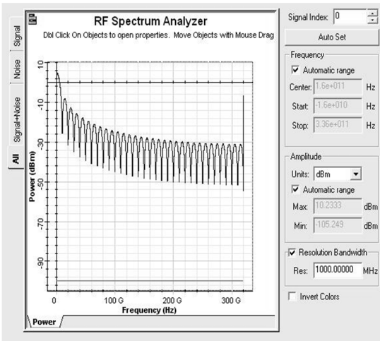
Fig 4(b). RF Spectrum Analysis for ROF using DPSK
