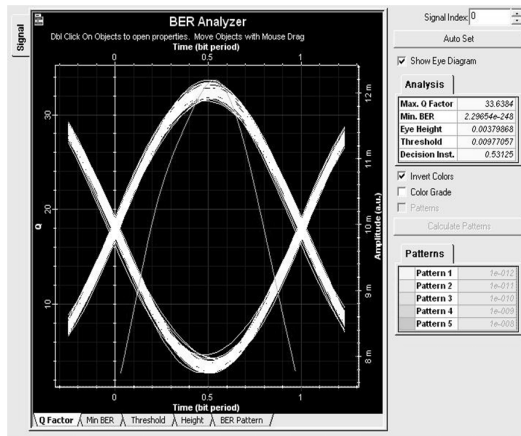
Fig 3(d). BER Analysis for ROF using CPFSK
