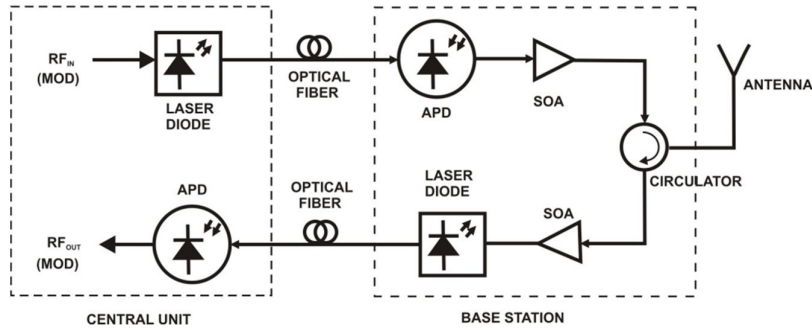
Fig 1. A Real-time ROF System
