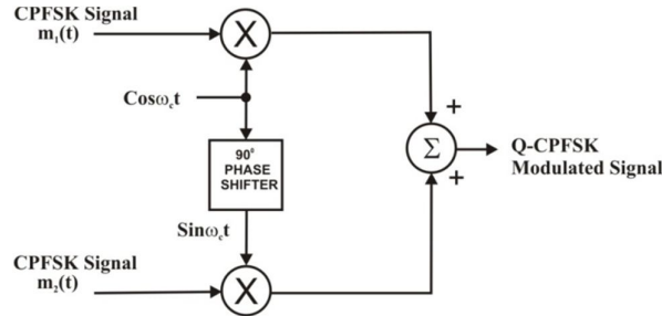
Fig 2(e) Quadrature Modulator
