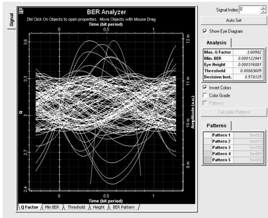
Fig 3(c). BER Analysis for ROF using OQPSK
