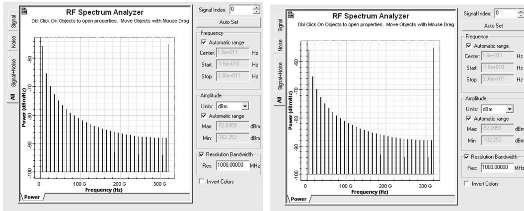
Fig 4(d). RF Spectrum Analysis for ROF using CPFSK
